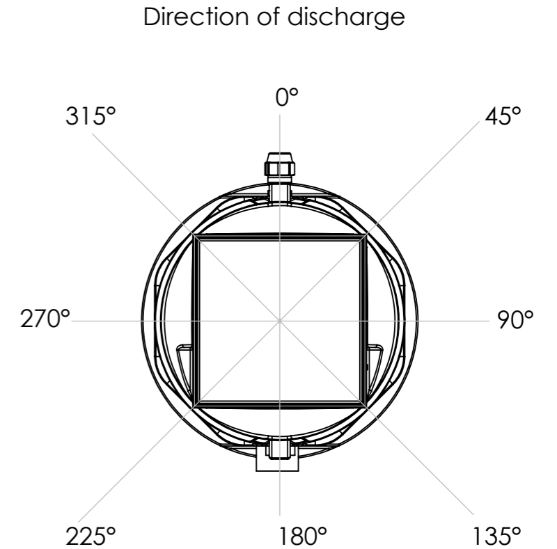
Inlet Orientation (Duct positioned @ 180°)
