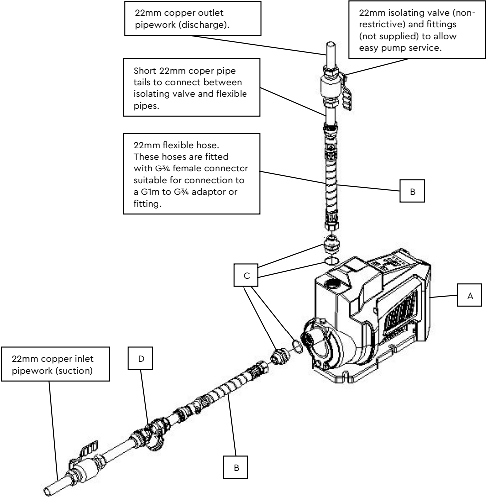
Fig 1. Typical installation configuration.
