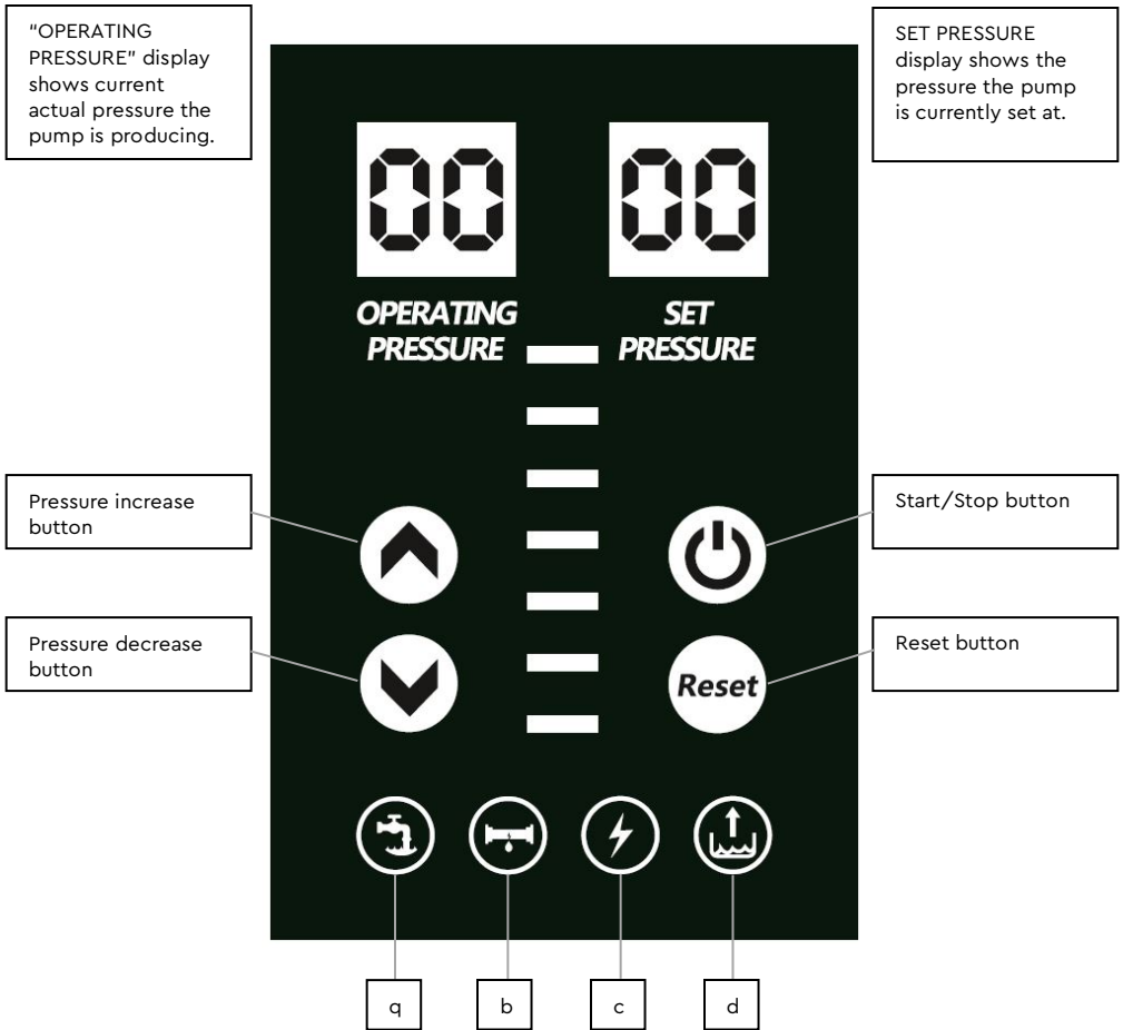
Fig 6. Control panel
