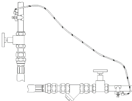
Fig 4. Diagram of earth continuity connections
